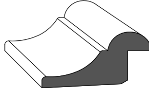
A-9 13/16" x 1-9/16" (1/2" inset)
