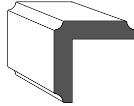
F-10 1-1/8" x 1-1/8"
