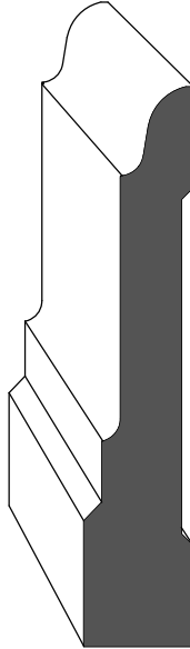
D-8 11/16" x 3-1/2"
