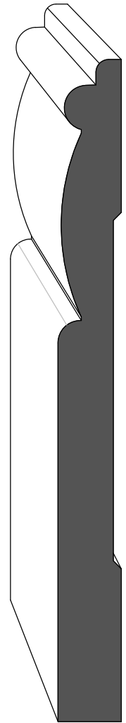
D-14 5/8" x 6-1/2"
