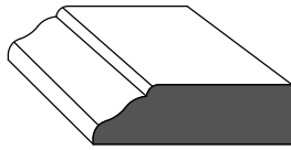
936 Stop 3/8" x 1-1/4"
